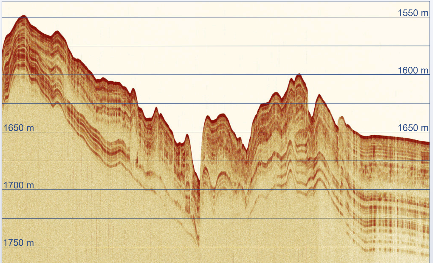
Innomar "deep-15" SBP data example (pulse 3 kHz, water depth c. 1600 m, penetration c. 100 m)
